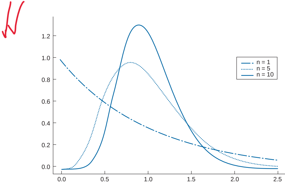
FIGURE 6.4 Densities of the average of n exponential random variables having mean 1.
